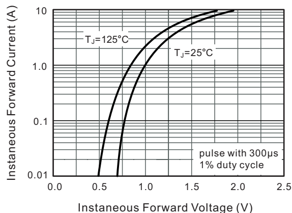
FIG.2-TYPICAL FORWARD CHARACTERISTICS
