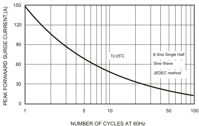
FIG.4-MAXIMUM NON-REPETITIVE FORWARD
