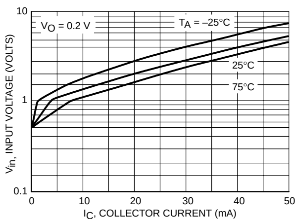
Figure 21. Input Voltage vs. Output Current
