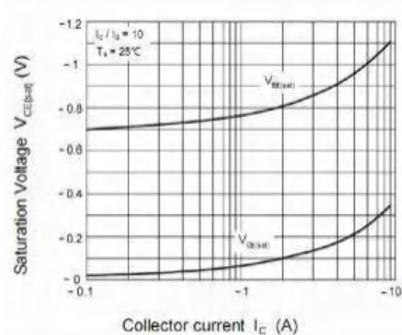
Figure 2 . Saturation Voltage
