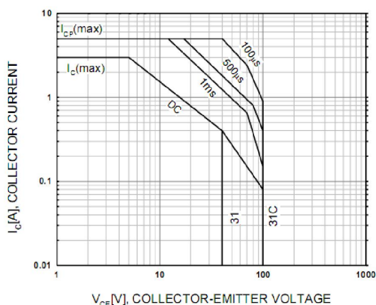
Figure 6. Safe Operating
