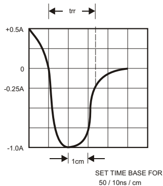
FIG.5 - TYPICAL REVERSE CHARACTERISTICS
