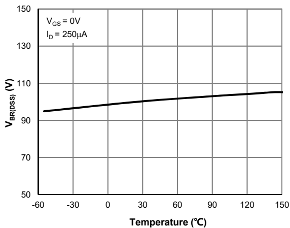
Figure 6: V_{BR(DSS)} vs. Junction Temperature
