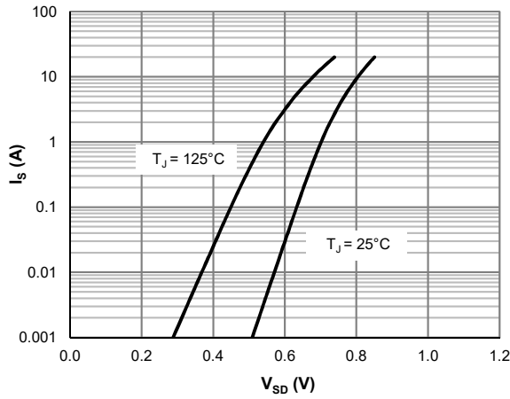
Figure 7: Body-Diode Characteristics
