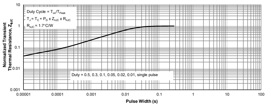
Figure 13: Normalized Maximum Transient Thermal Impedance
