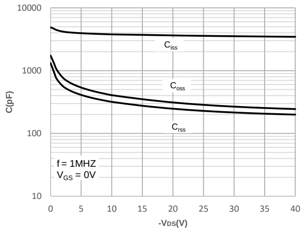
Figure 10: Capacitance Characteristics
