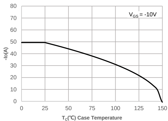
Figure 2: Current De-rating
