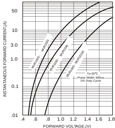
FIG.2-TYPICAL FORWARD CHARACTERISTICS
