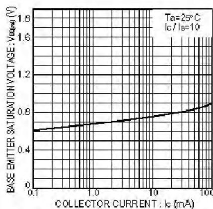
Fig.9 Base-emitter saturation voltage vs. collector current
