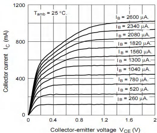
Figure 1. Static Characteristic
