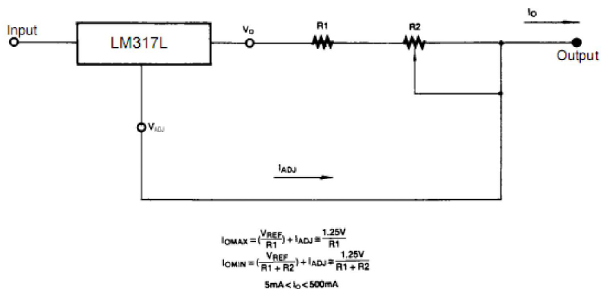
Figure 3.Current Regulator
