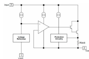
Internal Block Diagram
