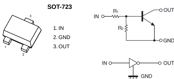
Equivalent Circuit
