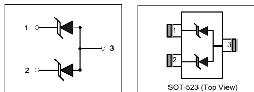
Schematic & PIN Configuration
