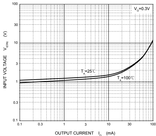
ON Characteristics
