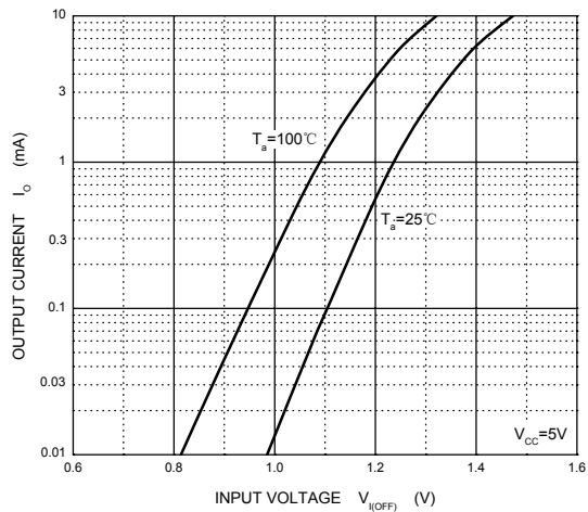
OFF Characteristics
