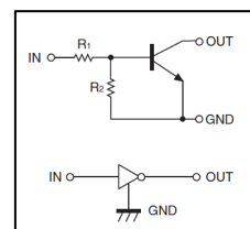
Equivalent Circuit
