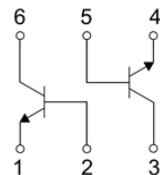
Equivalent Circuit
