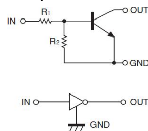
Equivalent Circuit
