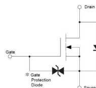
Equivalent Circuit
