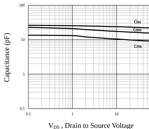
Fig.4 Capacitance Characteristics
