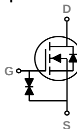
Equivalent Circuit
