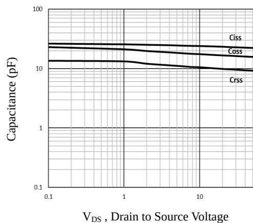
Fig.4 Capacitance Characteristics
