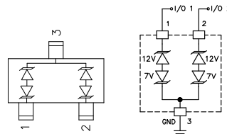
Schematic & PIN Configuration
