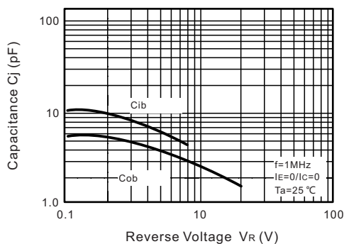
Fig.8 Cob/Cib--Vcb/VEB
