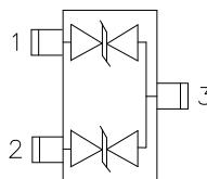
Circuit and Pin Schematic
