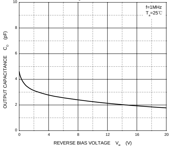
C_O — V_R
