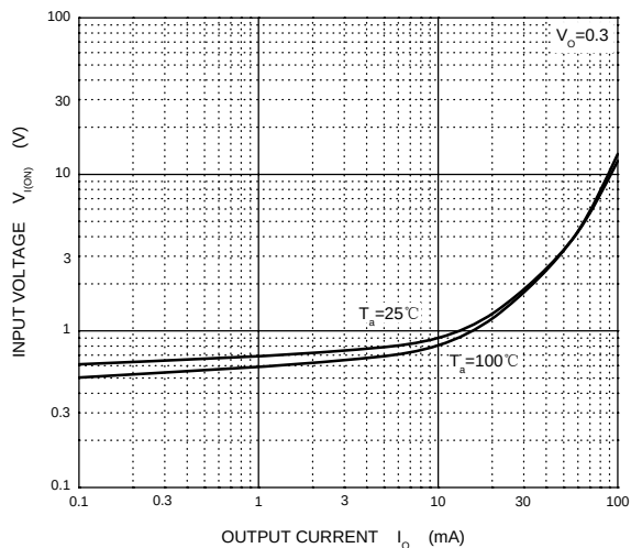
ON Characteristics
