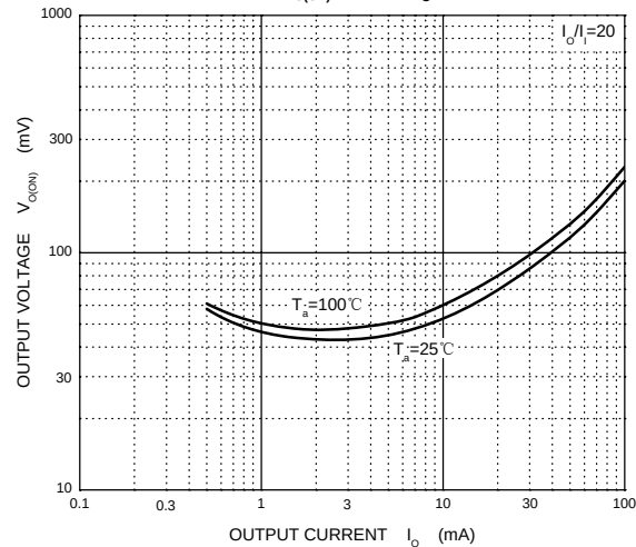
V_{O(on)} — I_O
