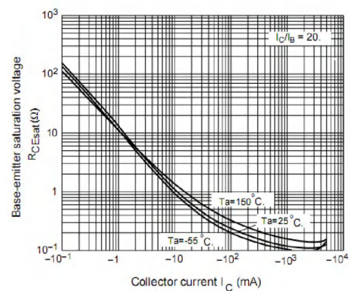
Figure 6. Equivalent on-resistance
