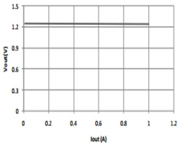
AMS1117-ADJ Vout Vs. Iout
