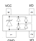
PIN Diagram
