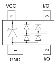
PIN Diagram
