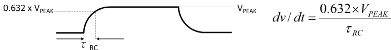
Fig.18 Waveforms of dV/dt
