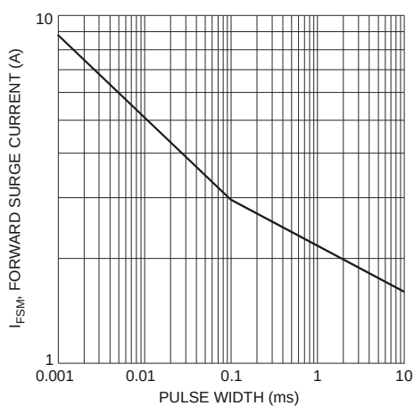
Fig. 5 Maximum Non-Repetitive Surge Currer
