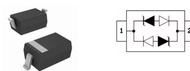
SOD-323
