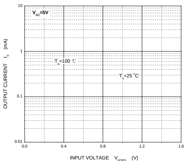
OFF Characteristics
