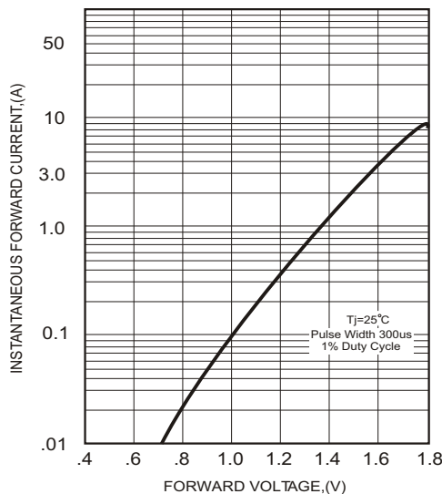
FIG.2-TYPICAL FORWARD CHARACTERISTICS
