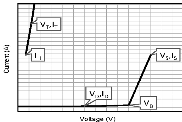
Figure 4: VI Curve
