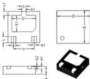
DFN2020-3L
