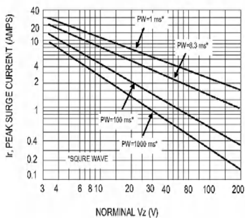
Maximum Non-Repetitive Surg Current versus Nominal Zener Voltage
