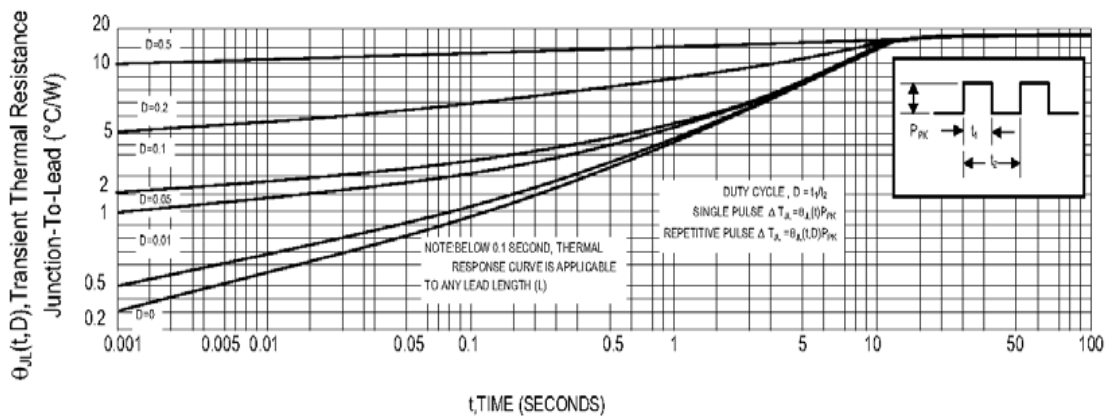
Typical Thermal Response L, Lead Length = 3/8 Inch
