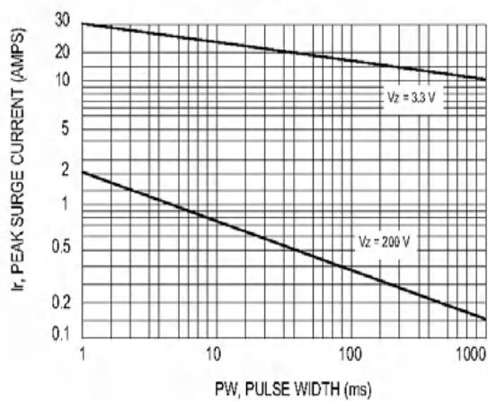
Peak Surg Current versus Pulse Width
