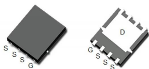
PDFN5X6-8L top&bottom view
