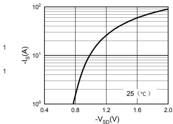
Figure 9. Body-Diode Characteristics
