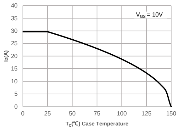
Figure 2: Current De-rating
