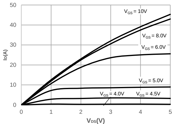
Figure 5: Output Characteristics
