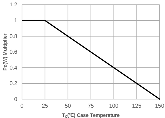
Figure 1: Power De-rating
