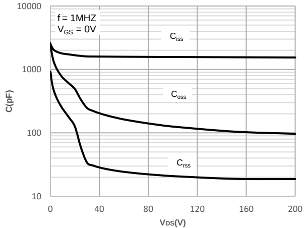
Figure 10: Capacitance Characteristics
