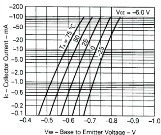
Fig.2 Collector Current vs. Base to Emitter Voltage
