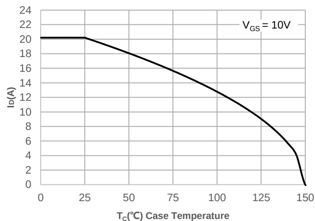
Figure 2: Current De-rating
