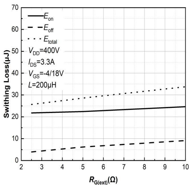
Figure 24. Clamped Inductive Switching Energy vs. R_{G(\text{ext})} T_j=175^{\circ}\text{C}
