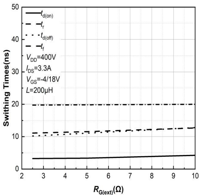
Figure 26. Switching Times vs. R_{G(ext)} T_J = 175^\circ\text{C}
