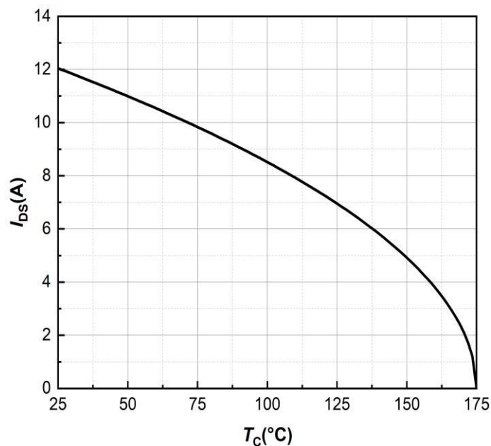
Figure 18. Continuous Drain Current Derating vs. Case Temperature
