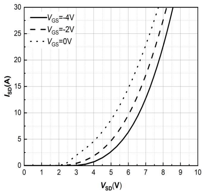
Figure 8. Body Diode Characteristic T_j = -40^\circ C
