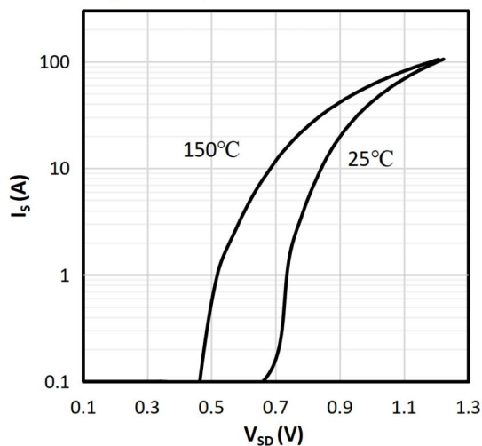
Fig 7: Body-Diode Characteristics
