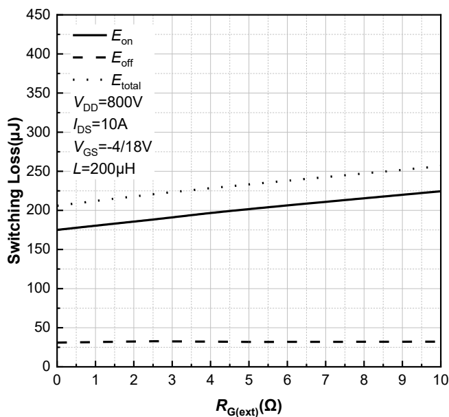
Figure 23. Clamped Inductive Switching Energy vs. R_{\text{G(ext)}} T_j = 25^\circ\text{C}
