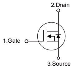
TO-247-3
