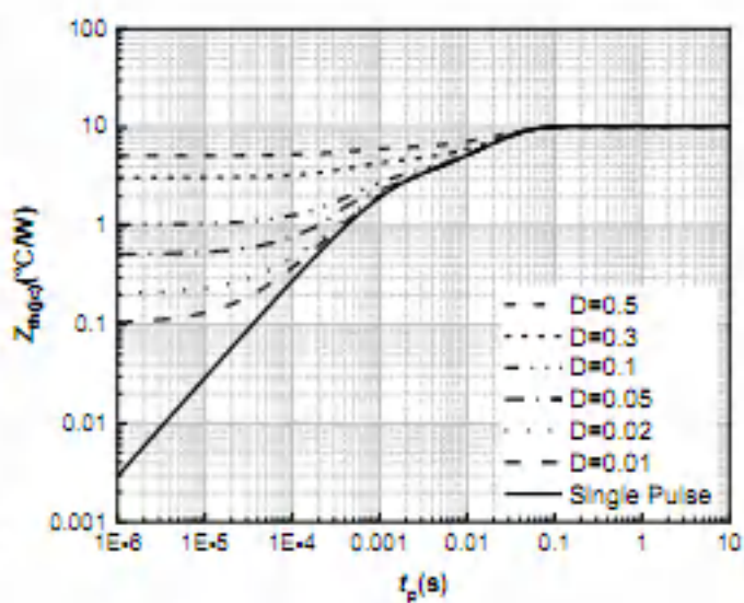
Figure 8. Max. transient thermal impedance, Z_{th(jt)} = f(t_p) , parameter: D = t_p / T
