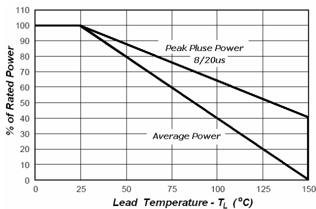
Fig3. Power Derating
