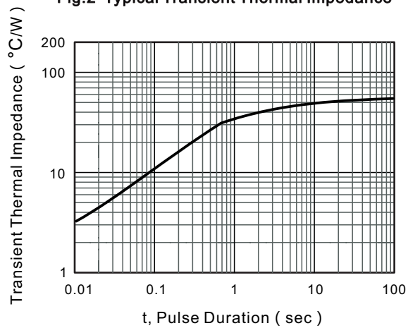
Fig.2 Typical Transient Thermal Impedance
