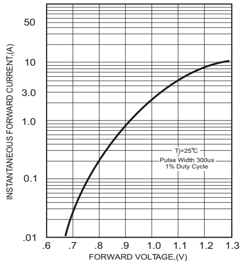
FIG.2-TYPICAL FORWARD CHARACTERISTICS
